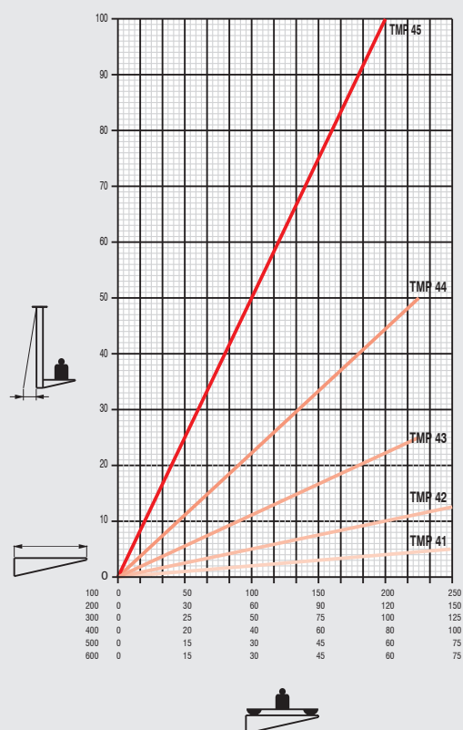
TMP 41-42-43-44-45 MAX. LOAD and DEFLECTION VALUES
