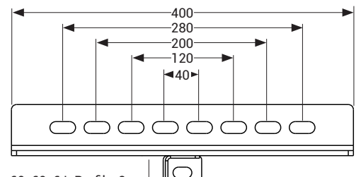
60x60x6 L Profile-2
