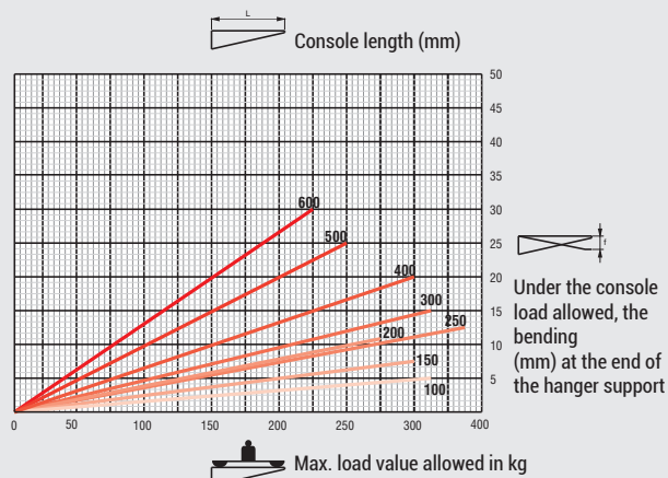
STS MAX. LOAD and DEFLECTION VALUES
