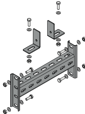
CCR/CR-UT Support Set ("T" boltless)
